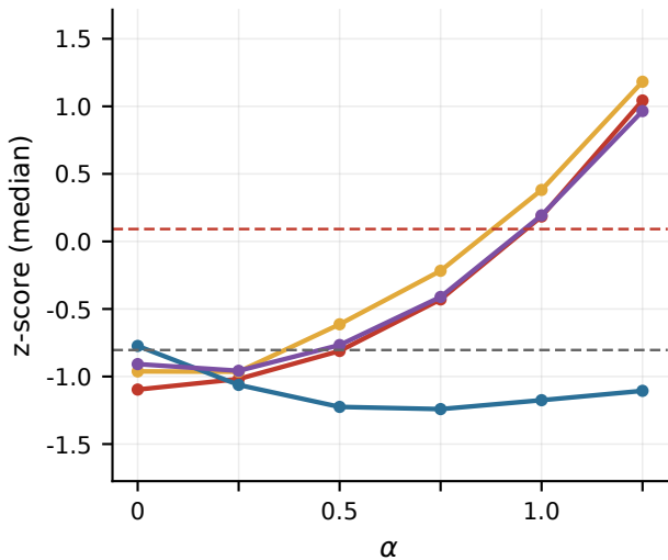
Loudness mean
